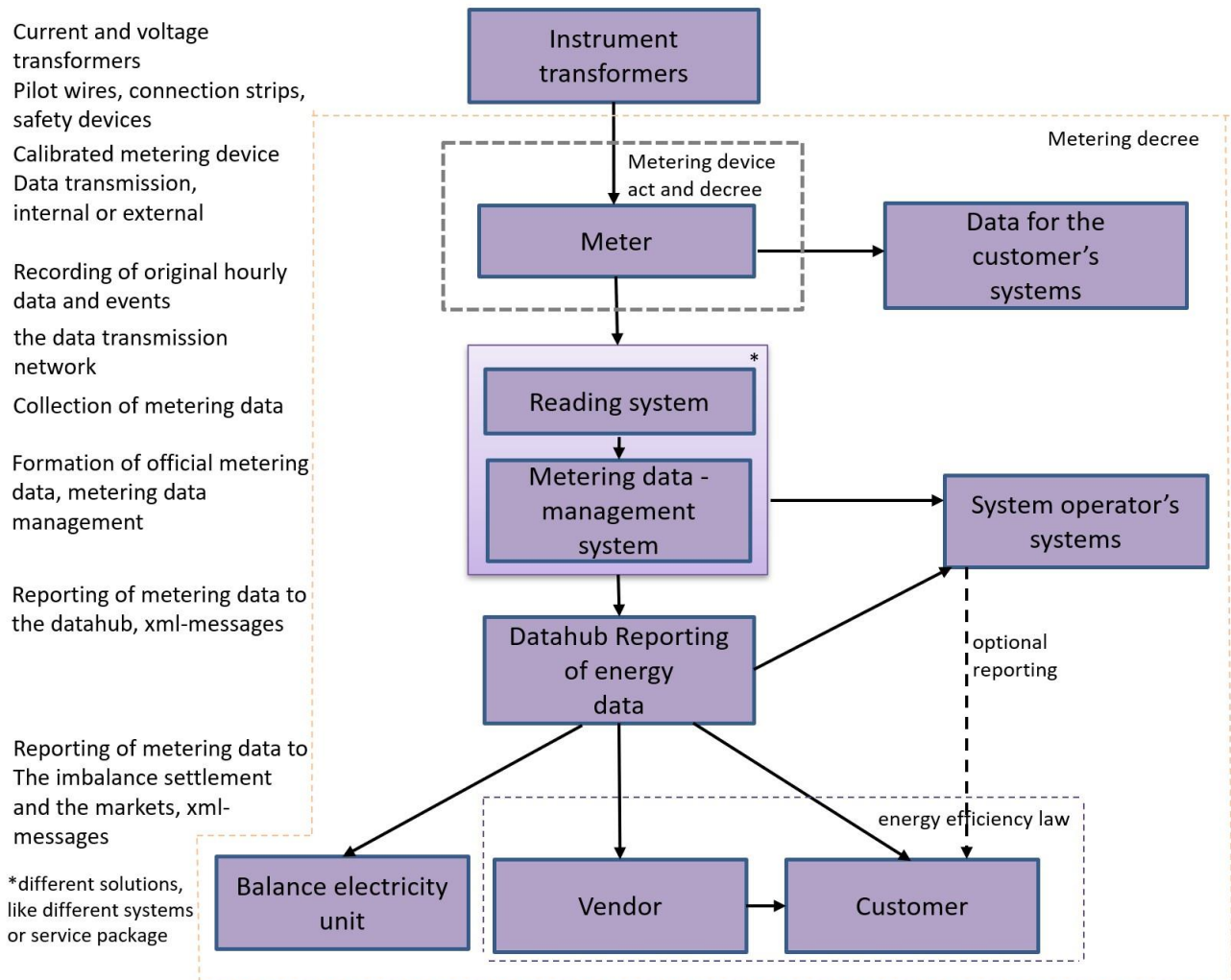
Figure 2. Metering and data transmission chain
