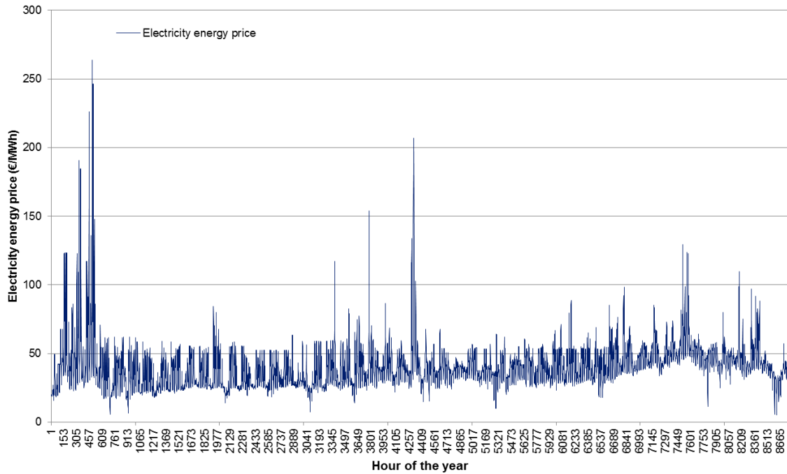
Figure 3-4 – Electricity energy price assumptions in the simulations
